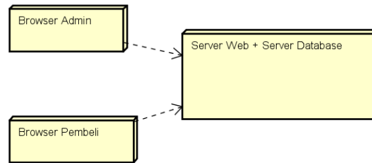
Gambar 7. Deployment diagram
