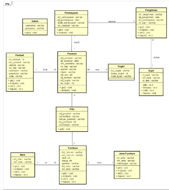
Gambar 6. Class diagram
